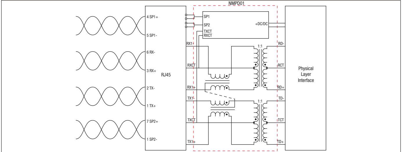
Figure 4 - Typical power coupling using the NMPD01
